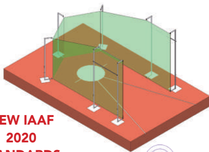
IAAF galvanized steel discus cage with ground sleeves Ref.13278
